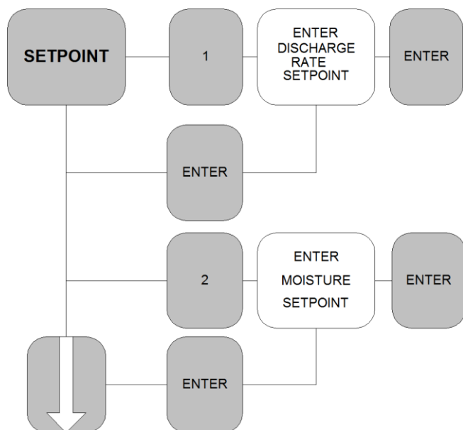
Figure 19 - Setpoint key hierarchy
