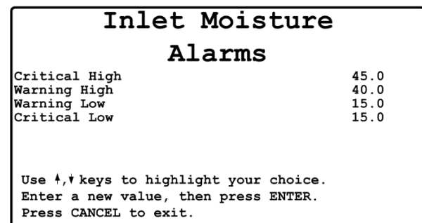
Figure 37- Inlet Moisture Alarms
