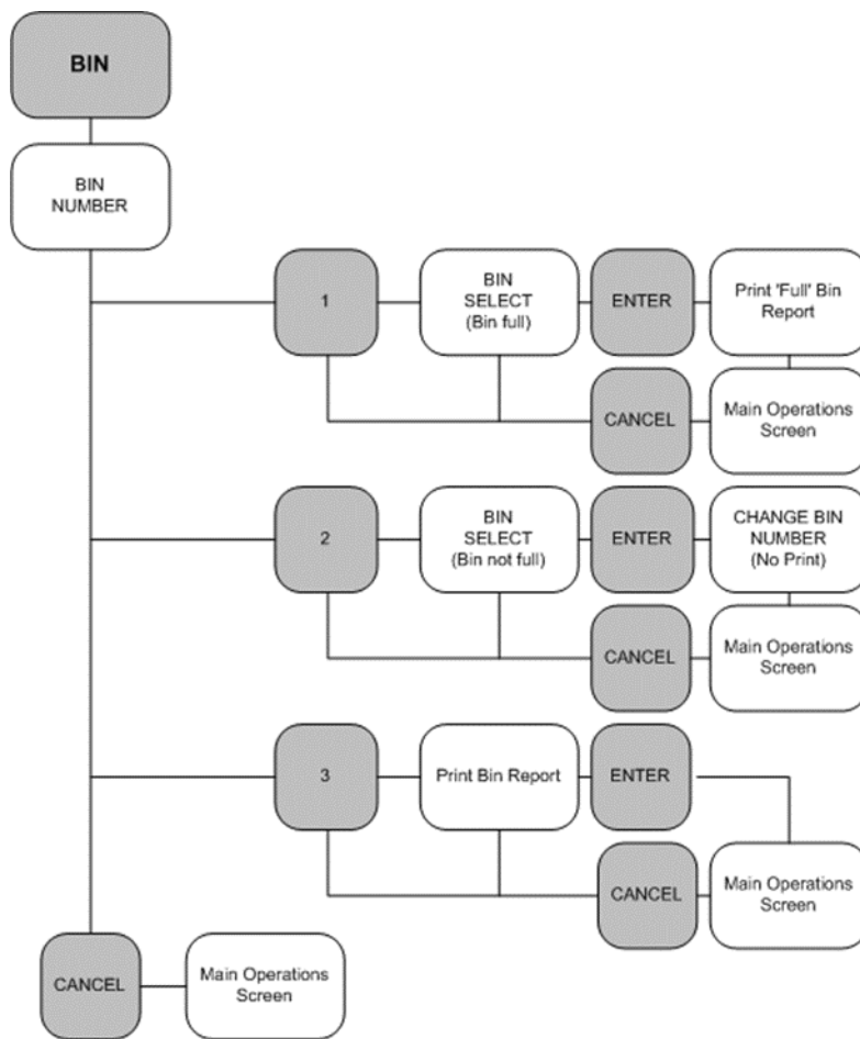
Figure 40- Bin key Hierarchy
