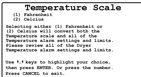
Figure 78 - Settings (Supervisor Setup) Temperature Scale menu
