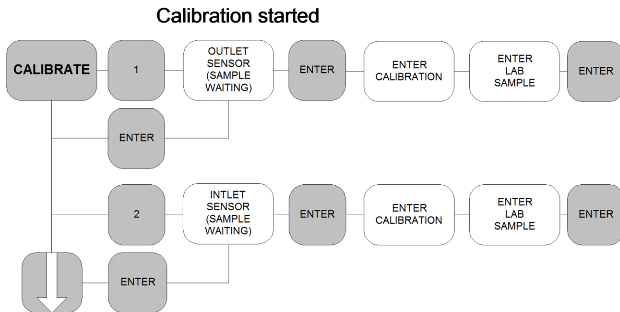
Figure 25 - Calibrate key hierarchy (calibration started)
