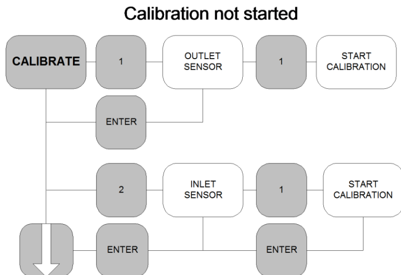
Figure 29 - Calibration not started hierarchy
