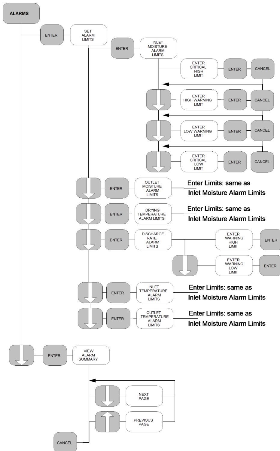
Figure 34 - Alarm key Hierarchy
