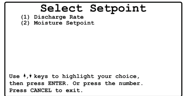
Figure 23 - Select setpoint menu (Moisture Setpoint)
