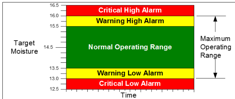
Figure 9 - Alarm Limit Operation
